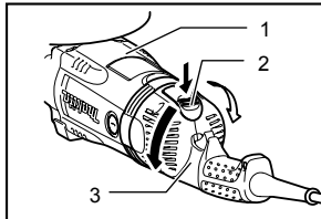
1. Motor housing 2. Lock button 3. Handle
