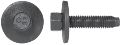
245-315 Std. Pkg. 25 pcs. M6-1.0x28mm FORD Body Bolt Phosphate Hex Head Sems® With Dog Point 19mm Washer O.D., Hex Size: 8mm #N606677-S43B CL Part No: 910-0060, Pieces: 4
