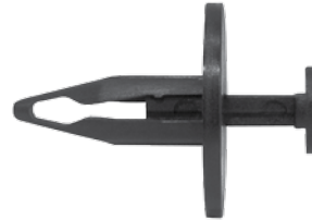
247-447 Std. Pkg. 25 pcs. Splash Shield Retainer FORD Splash Shield, Seat Cushion & Spare Tire Retainer Head Dia. 1", Stem L. 7/8", Fits into 5/16" Hole #N804614-S CL Part No: 910-0555, Pieces: 2
