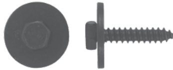
245-400 Std. Pkg. 25 pcs. M4.2-1.41x20mm GM Indented Hex Head Sems Phosphate 16mm Washer O.D., Hex Size: 7mm #11500434, 11503892, 1640810 CL Part No: 910-0030, Pieces: 5
