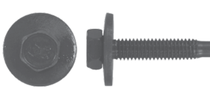
245-325 Std. Pkg. 25 pcs. M6-1.0x30mm CHRYSLER Body Bolt Phosphate 19mm Washer O.D., Hex Size: 10mm #6100568
