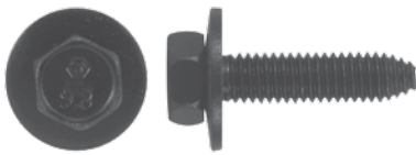
245-407 Std. Pkg. 25 pcs. M6-1.0x25mm GM Body Bolt Phosphate 17mm Washer O.D., Hex Size: 10mm #11503834, 20351035 CL Part No: 910-0050, Pieces: 5
