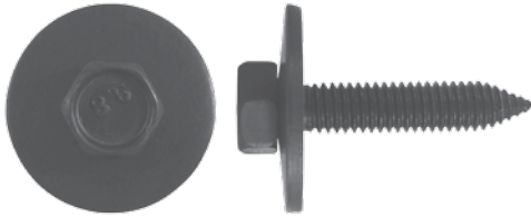
245-324 Std. Pkg. 25 pcs. M6-1.0x30mm GM Hex Head Sems® 24mm Washer O.D., Class 9.8, Hex Size: 10mm #11503825
