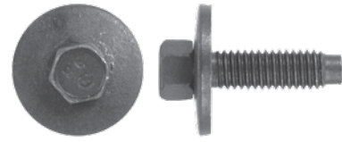
245-323 Std. Pkg. 25 pcs. M6-1.0x28mm FORD Hex Head Sems® With Dog Point 19mm Washer O.D., Class 9.8, Hex Size: 8mm #N606677-S36 CL Part No: 910-0057, Pieces: 3
